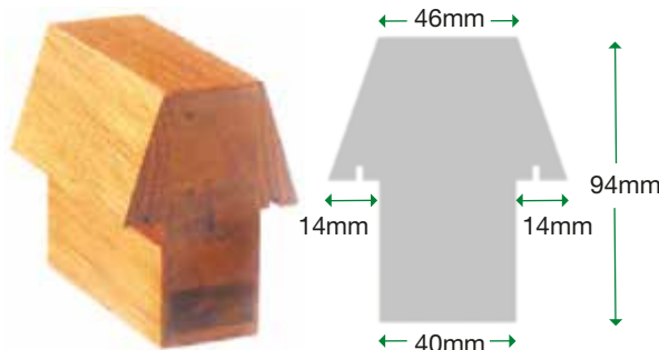
MULLION (DOUBLE REBATE)
